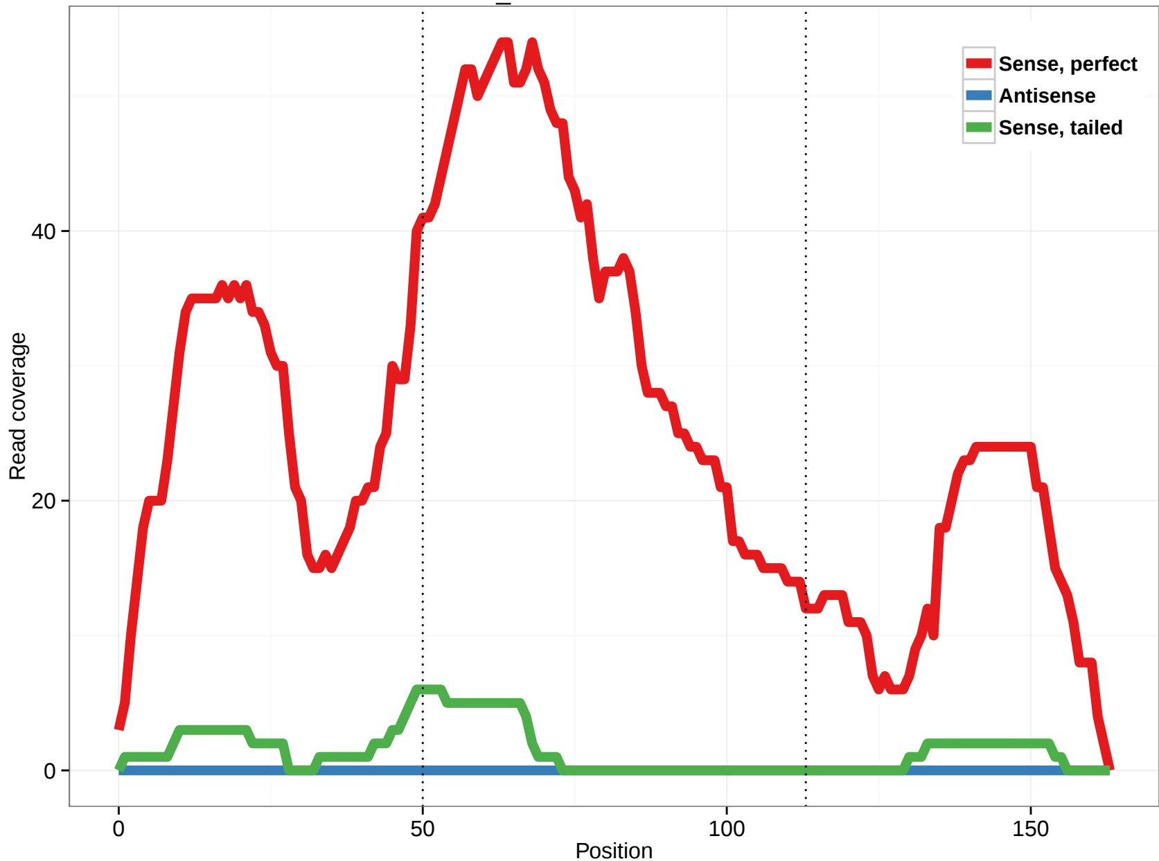
scaffold_4784:14078740-14078903
