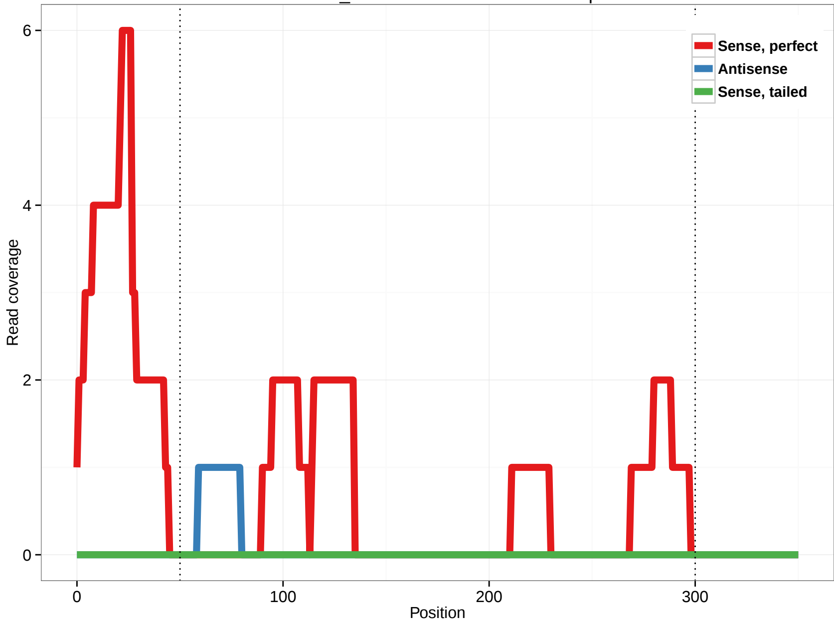
scaffold_4784:13845649-13849025.5p
