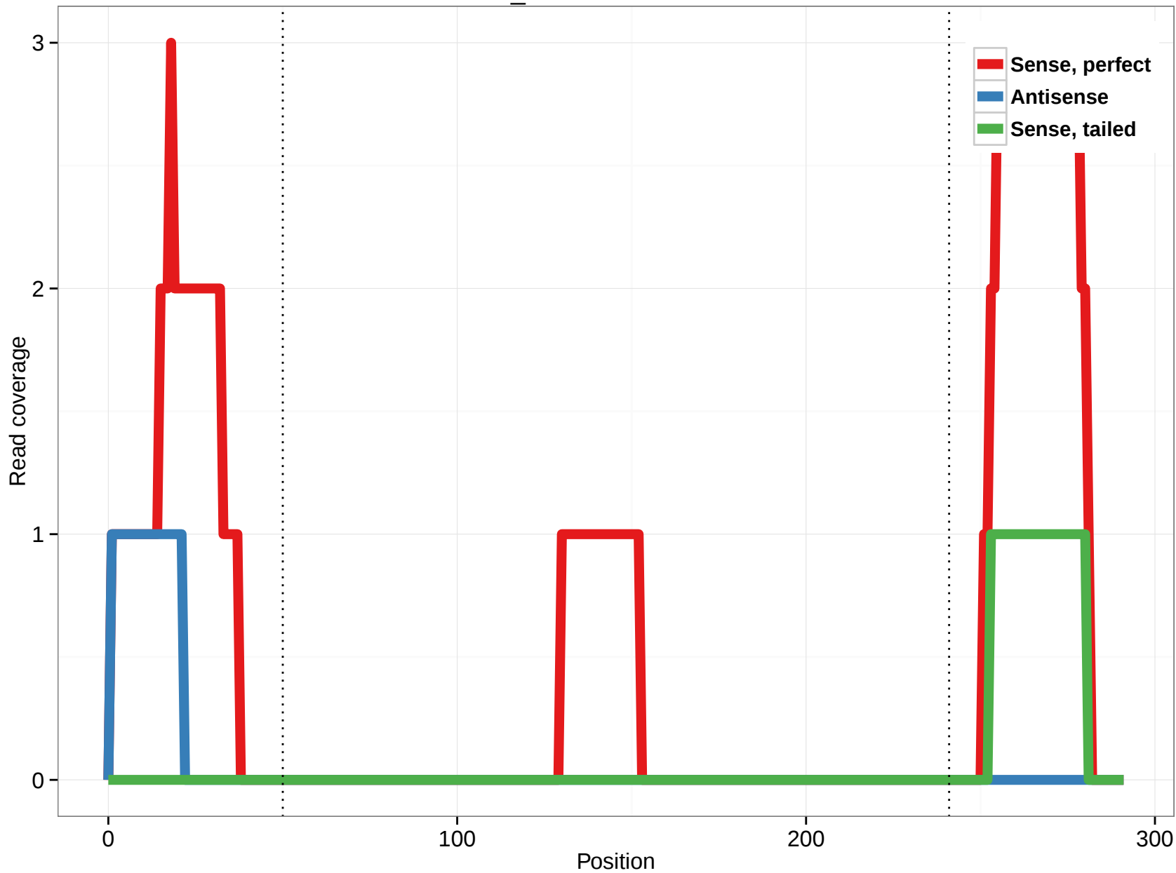
scaffold_4770:6223559-6223850
