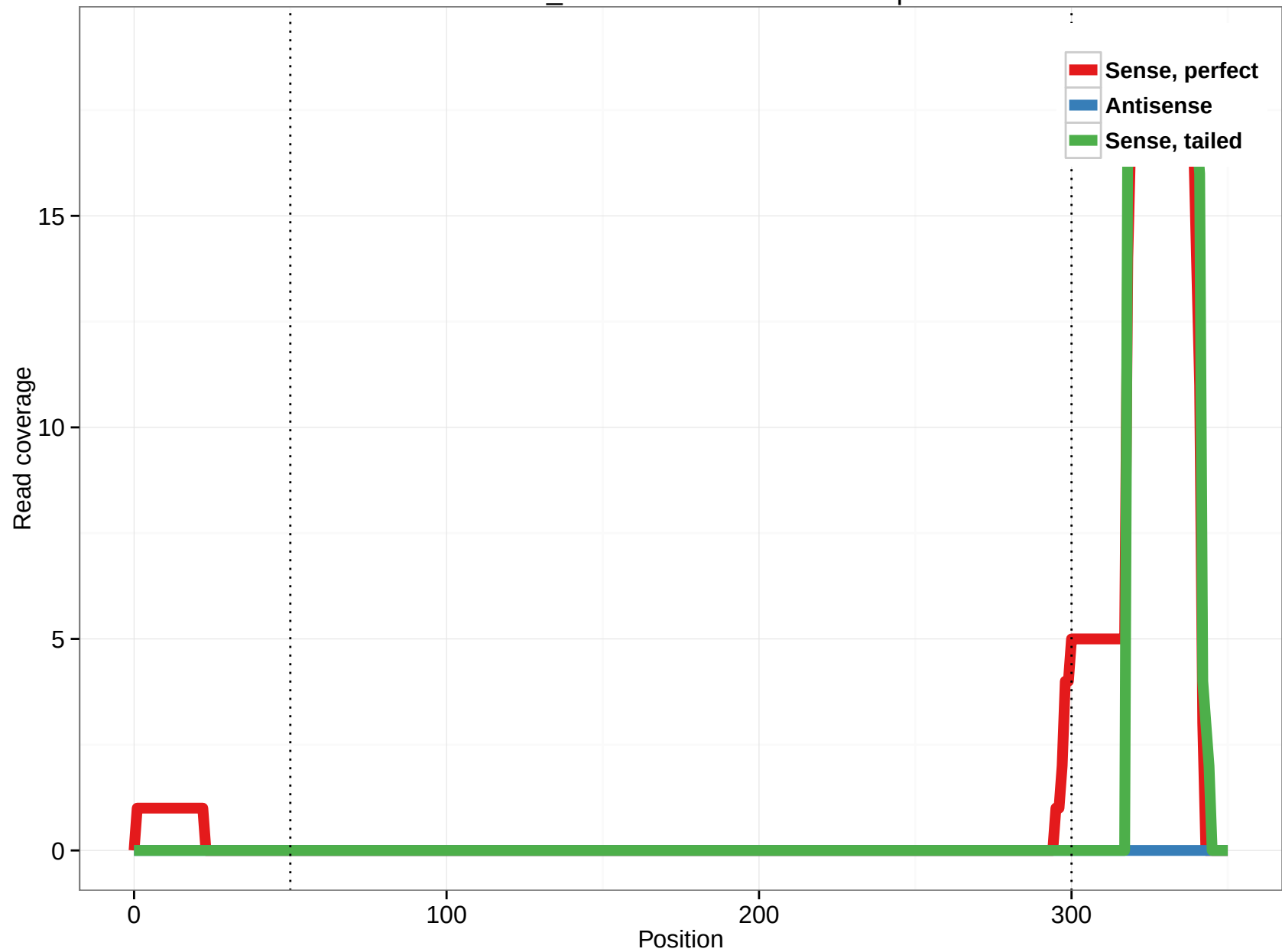
scaffold_4770:4216871-4218064.5p
