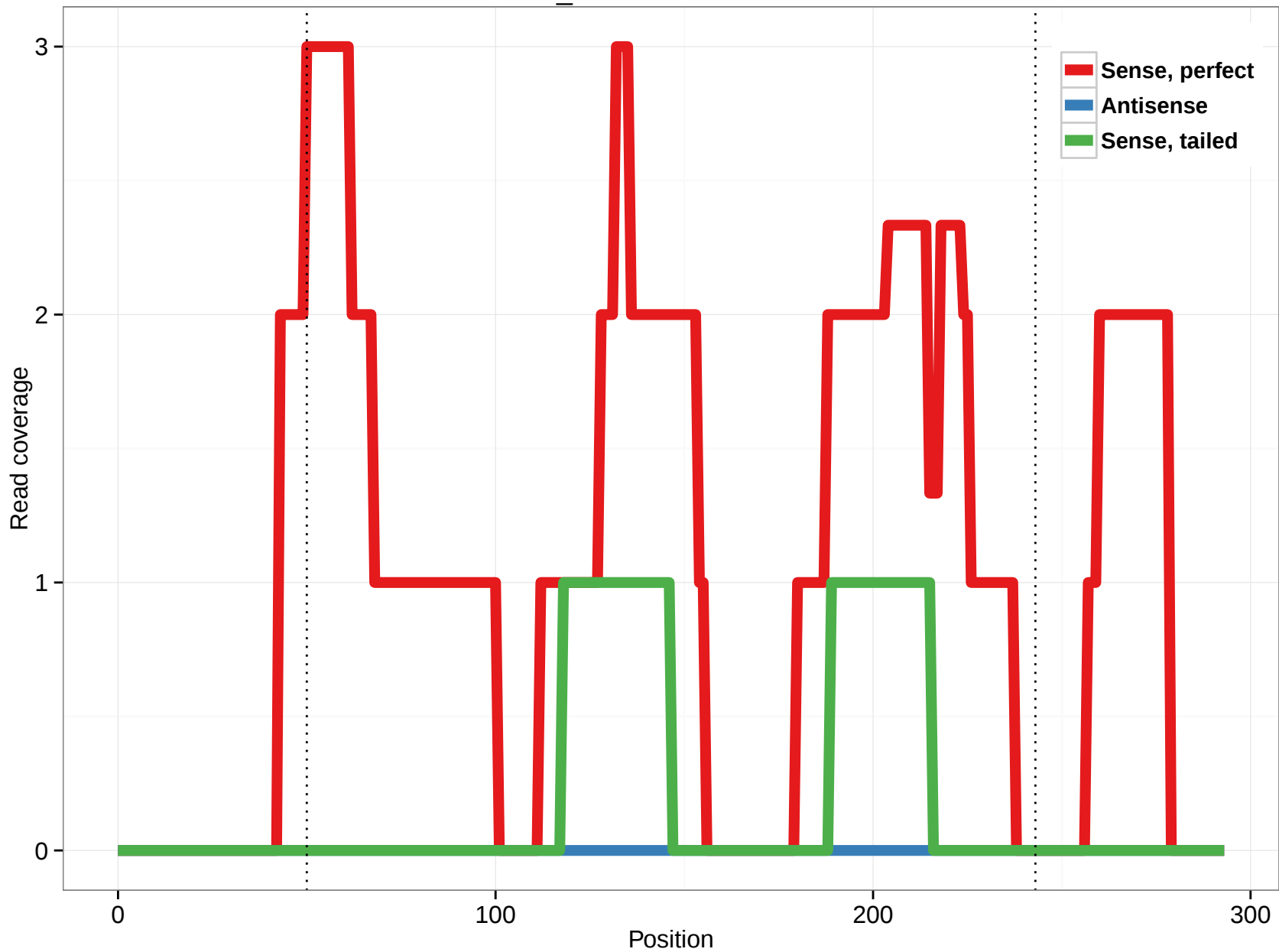
scaffold_4770:1696335-1696628
