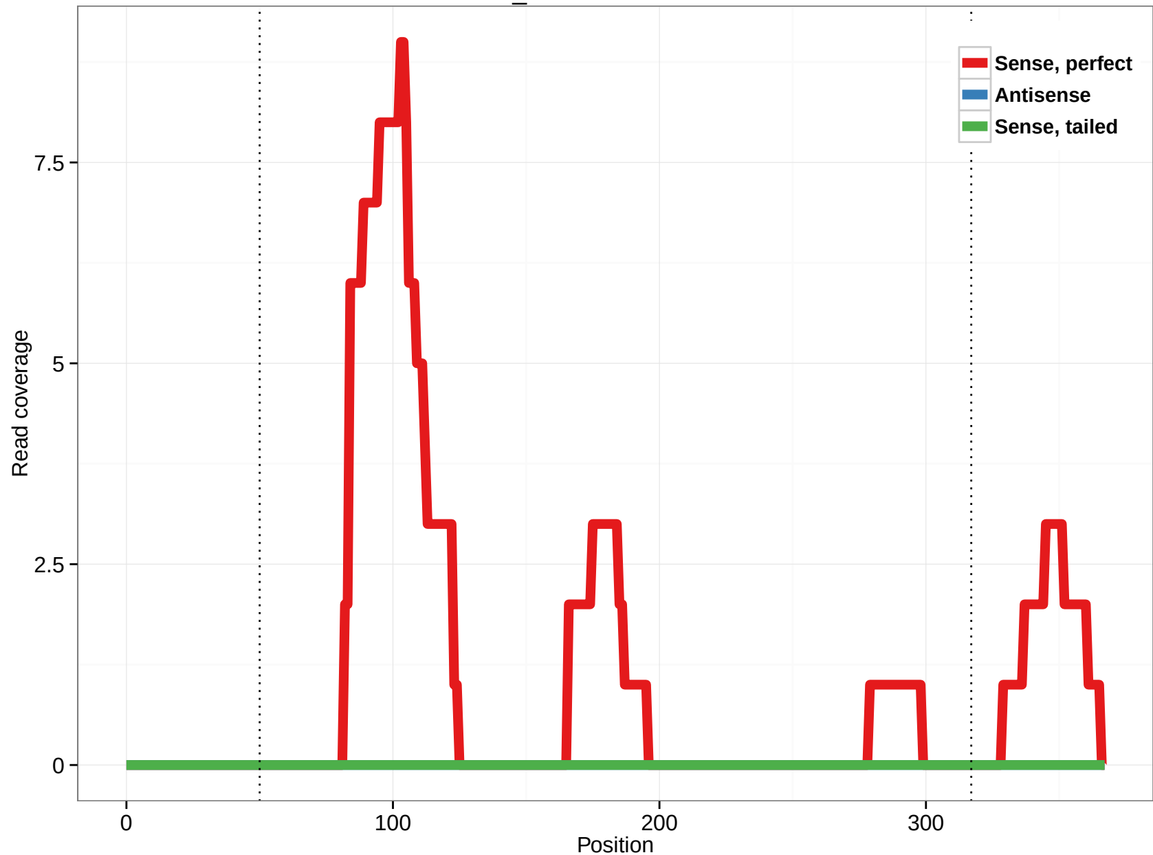
scaffold_4770:1654253-1654620
