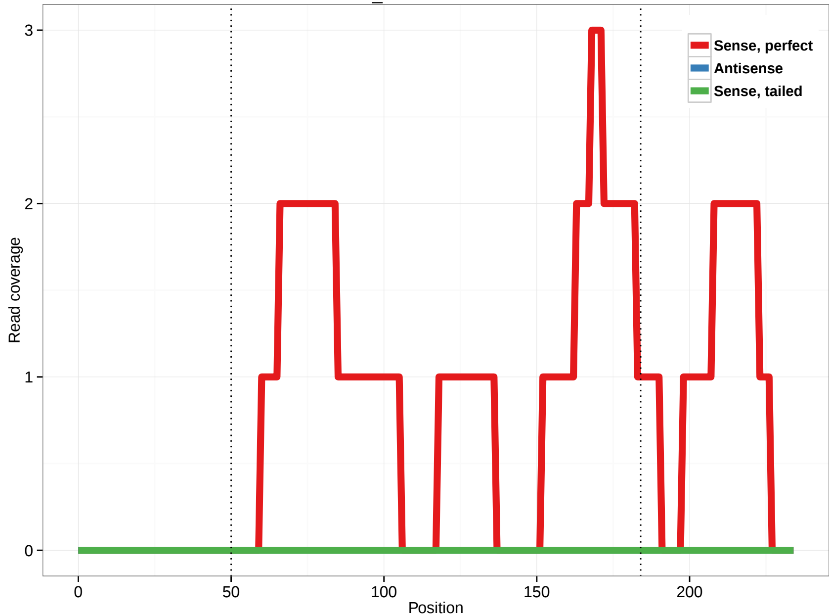
scaffold_4770:158213-158447
