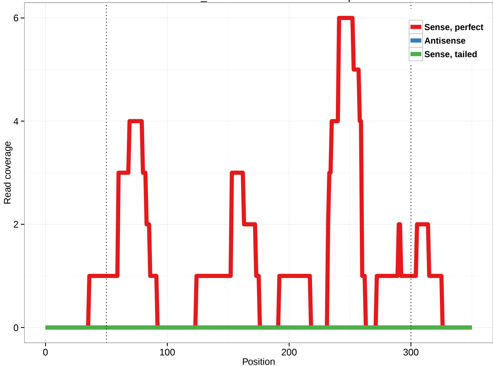
scaffold_4770:11623291-11624726.3p
