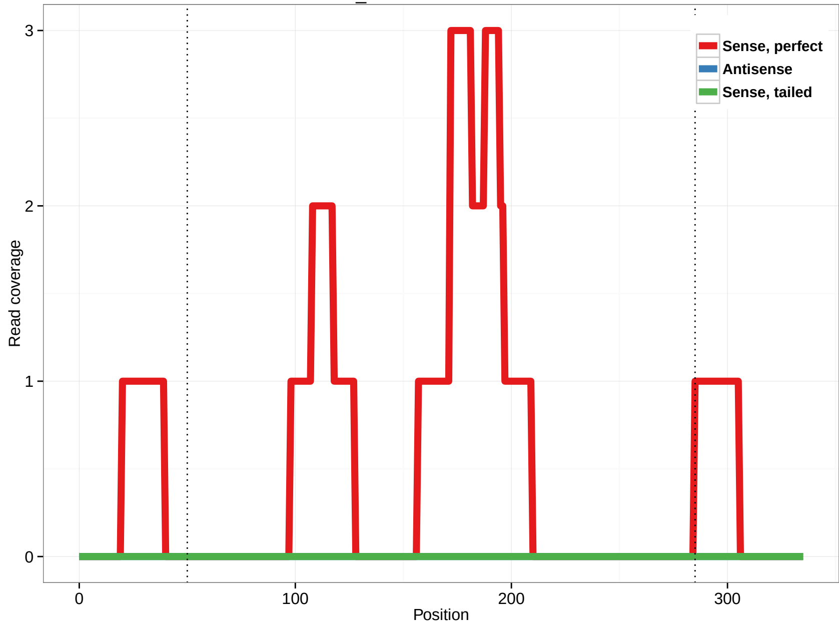
scaffold_4770:11403995-11404330
