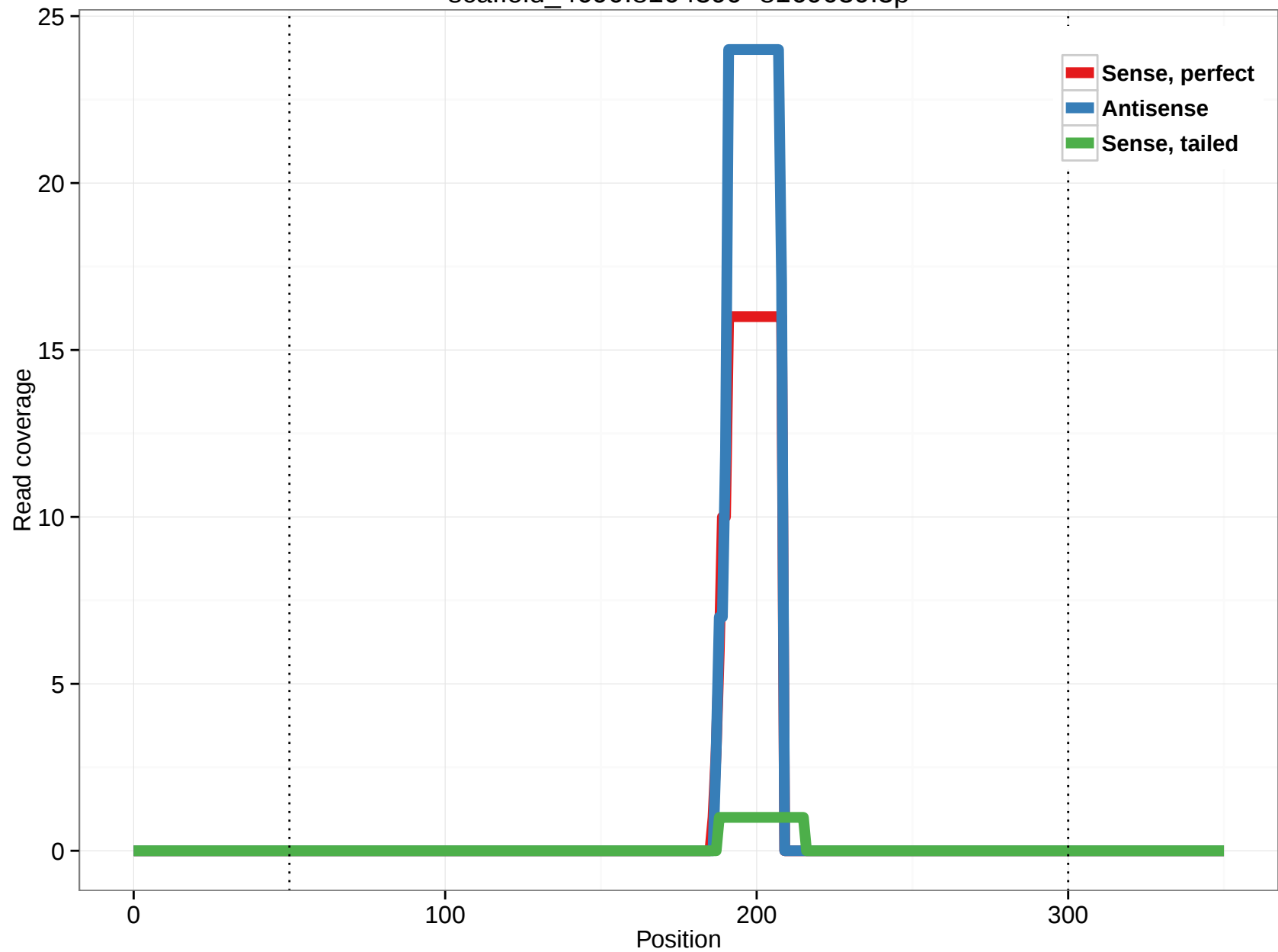
scaffold_4690:8164399-8169039.3p
