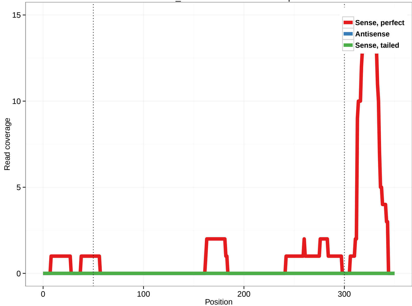
scaffold_4690:6708200-6709372.5p
