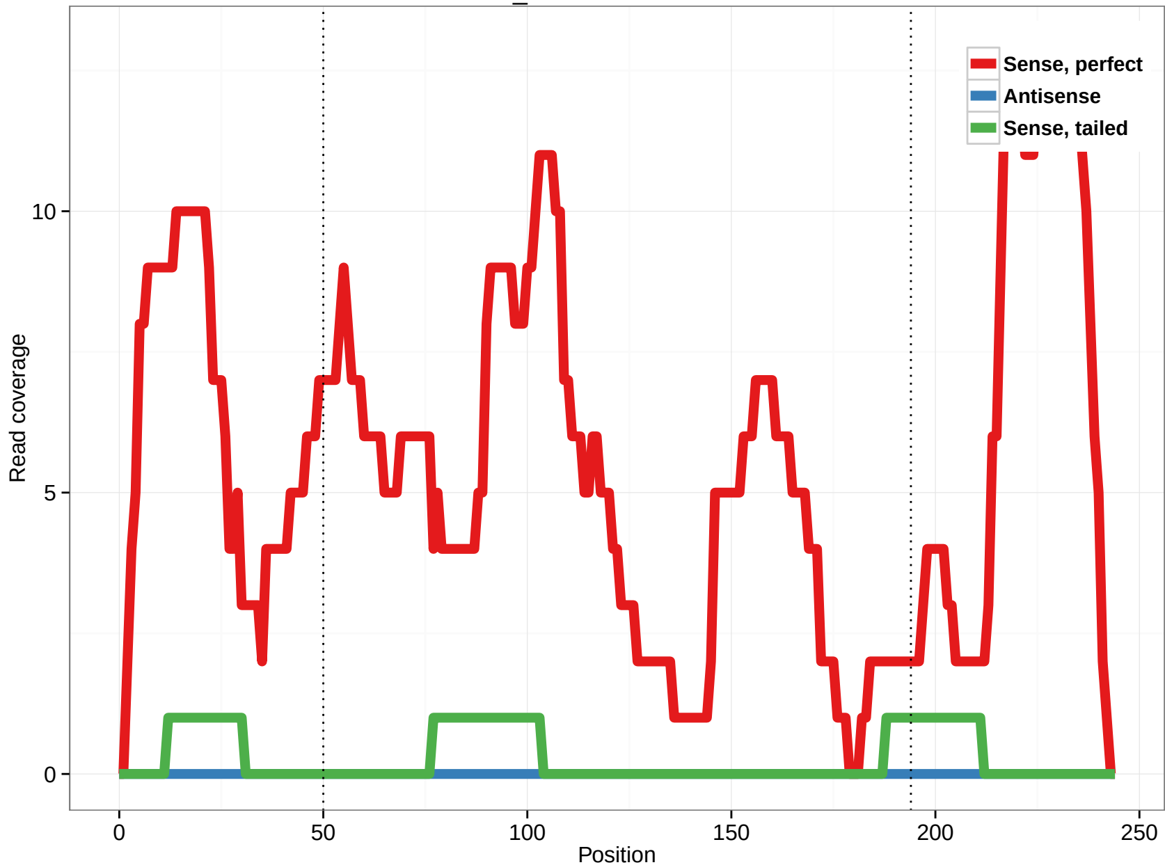
scaffold_4690:5158781-5159025
