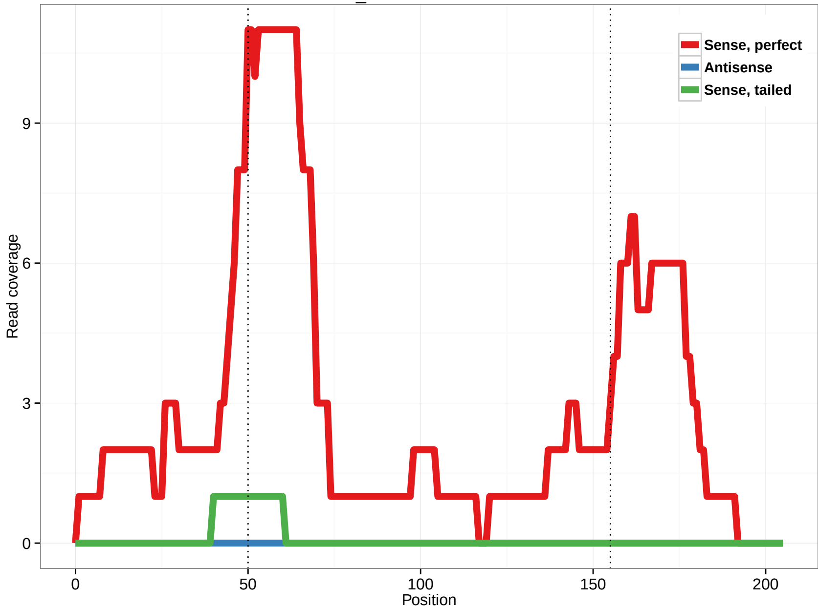
scaffold_4690:3442553-3442758
