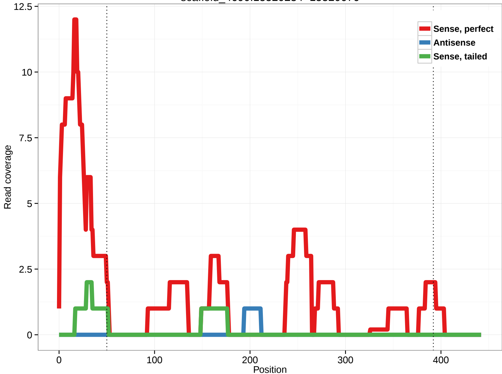
scaffold_4690:15520234-15520676
