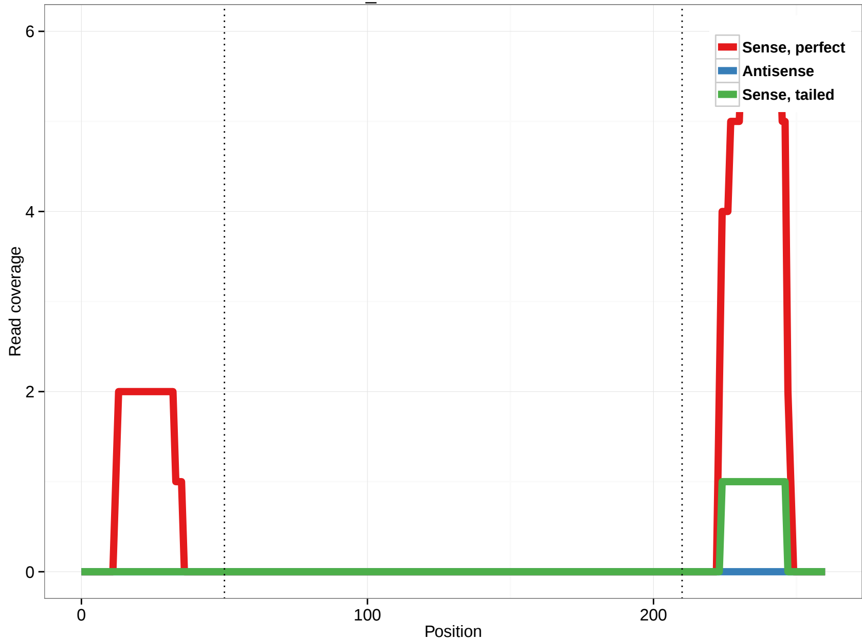
scaffold_4690:10179055-10179315
