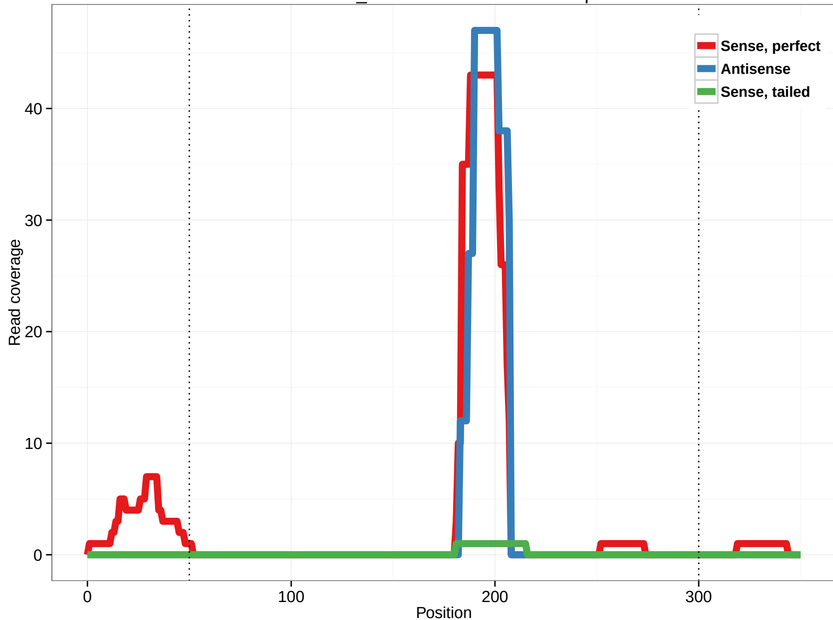
scaffold_4644:2511088-2512234.5p
