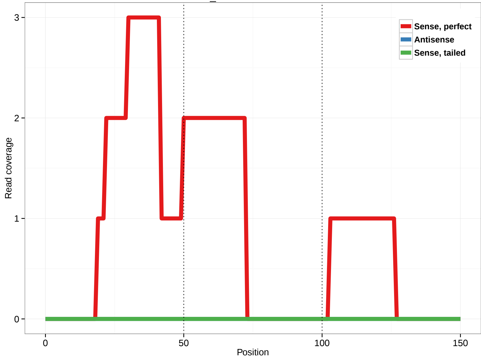
scaffold_4644:2061795-2061945
