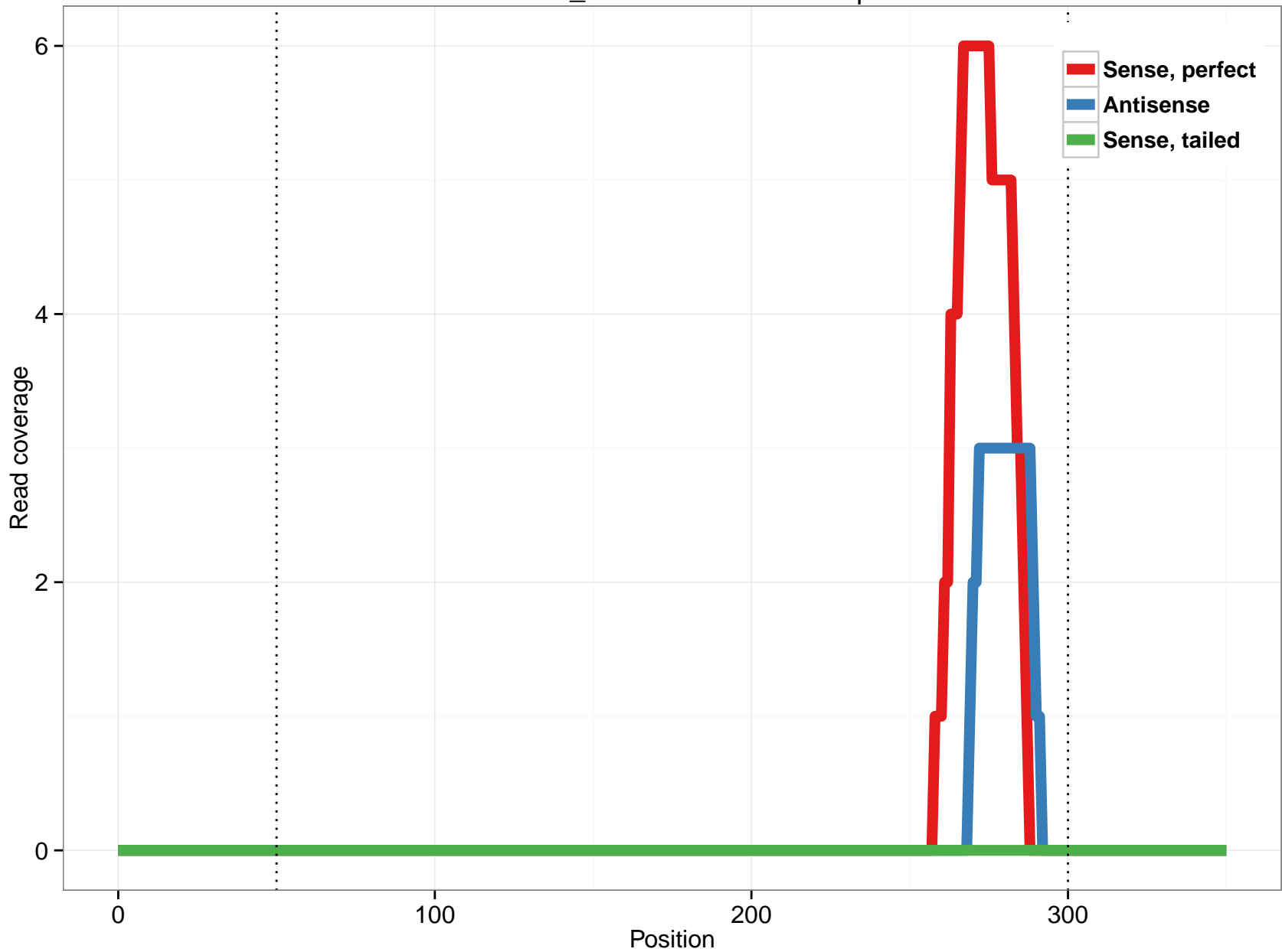
scaffold_4512:84686-85783.5p
