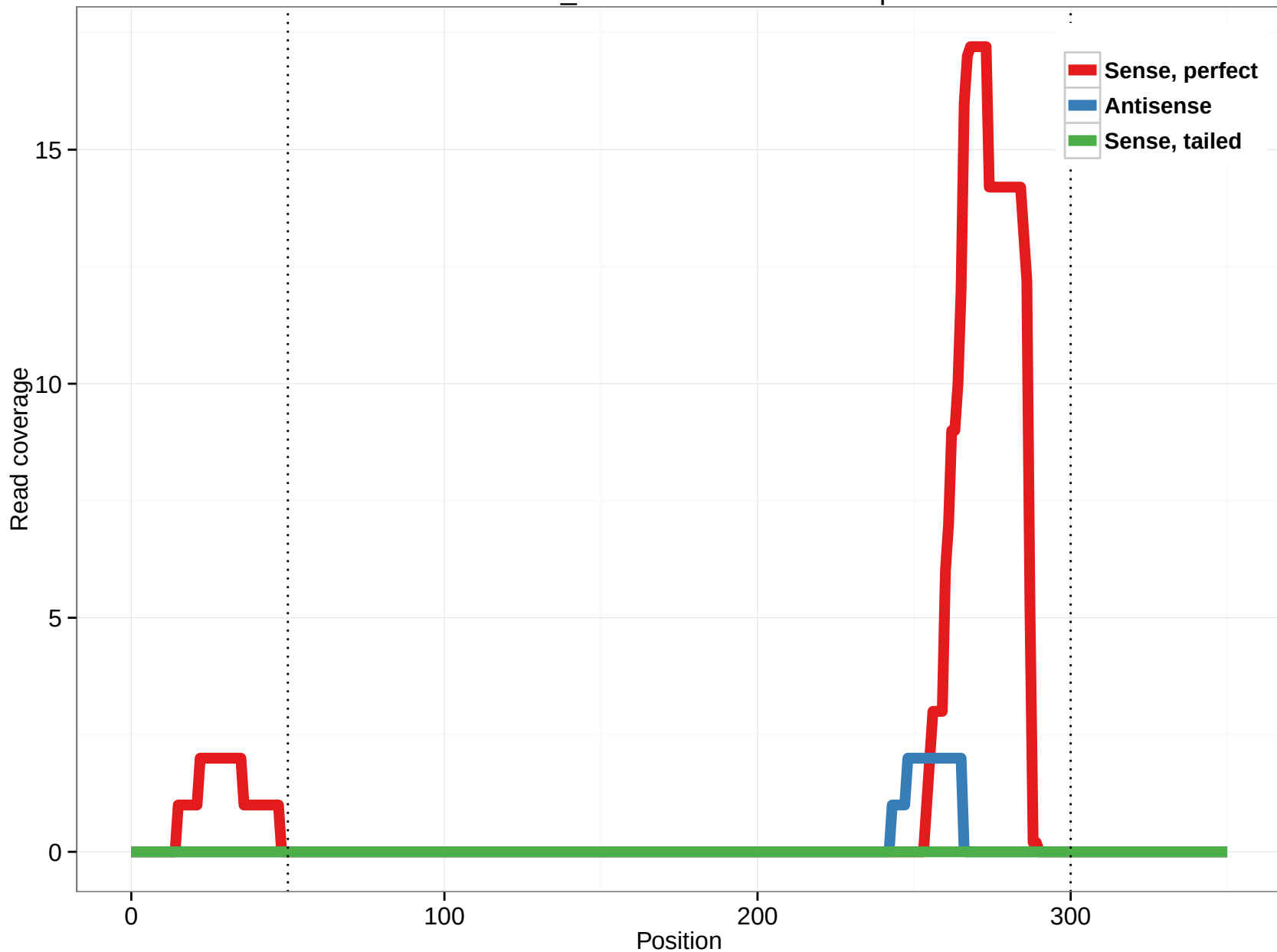
scaffold_4512:628453-630000.5p
