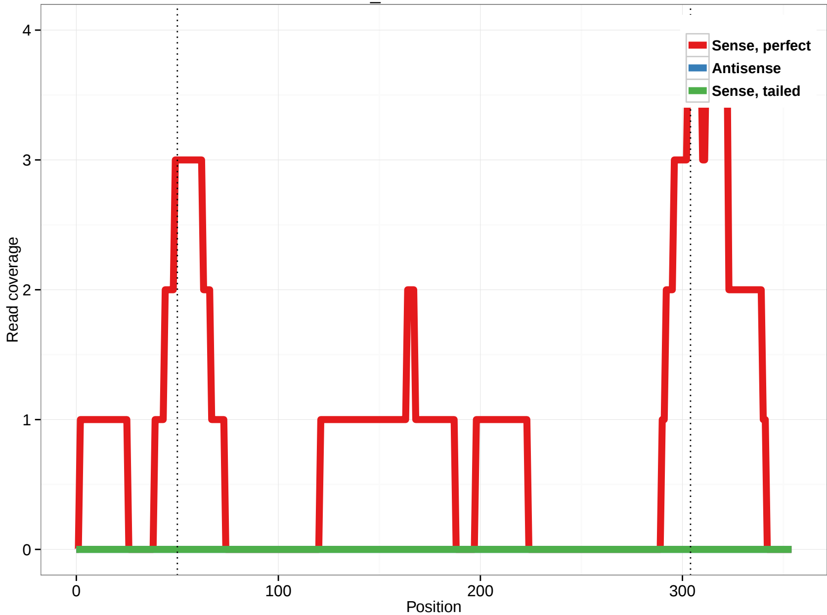
scaffold_4512:301079-301433
