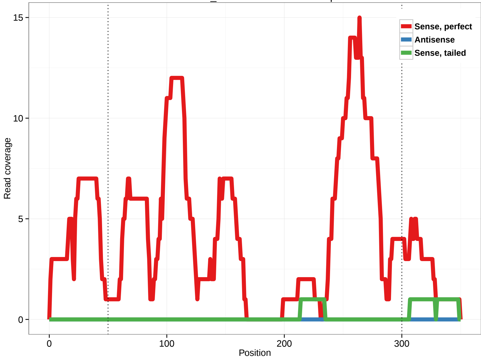
scaffold_4512:167705-168849.5p
