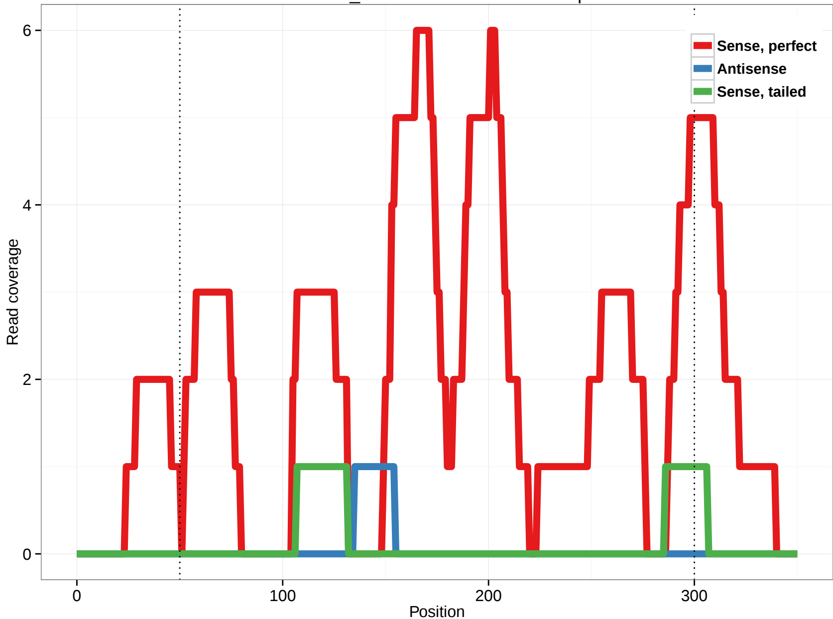
scaffold_4512:1169124-1170167.3p
