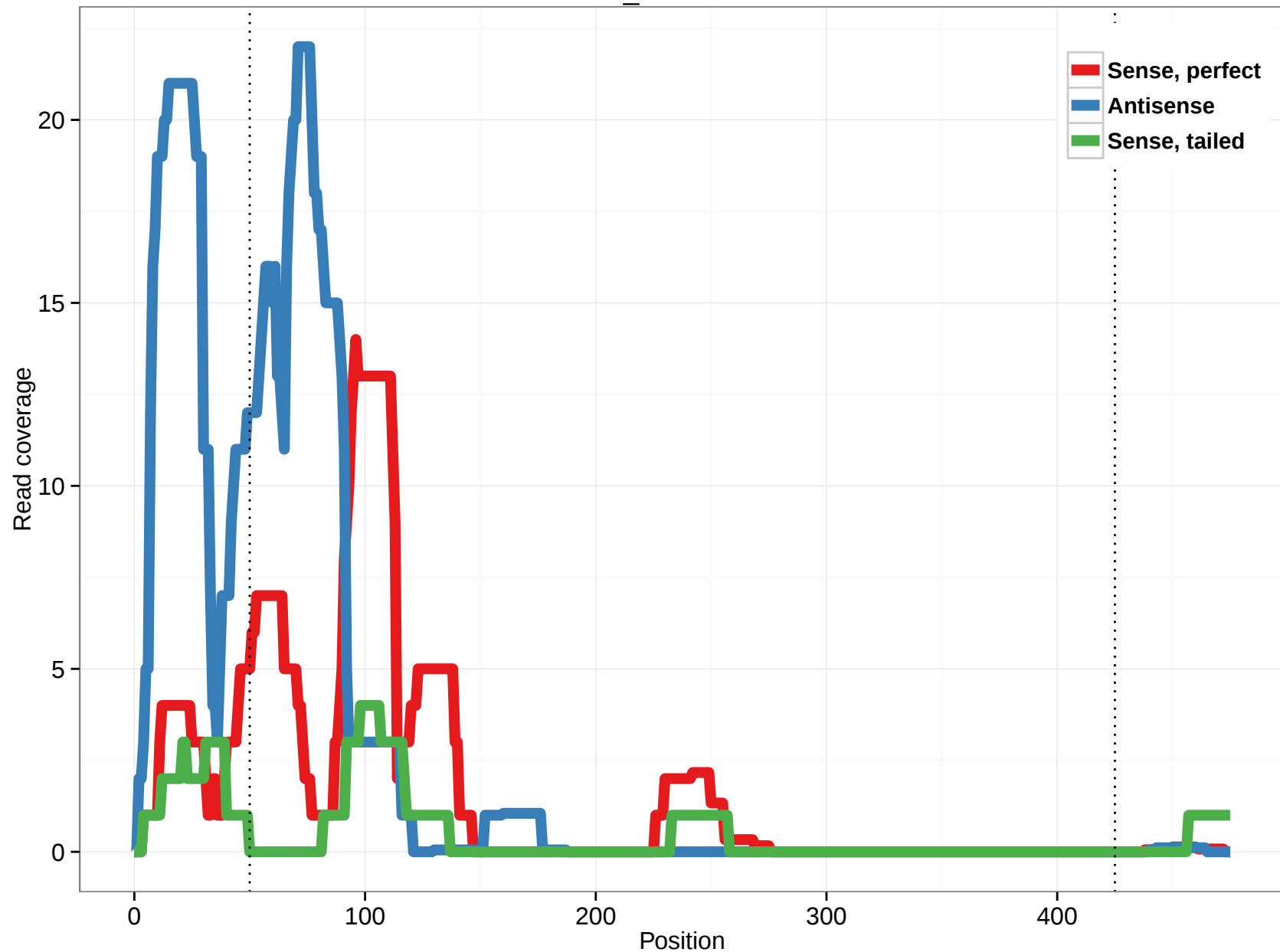
scaffold_3522:570-1045
