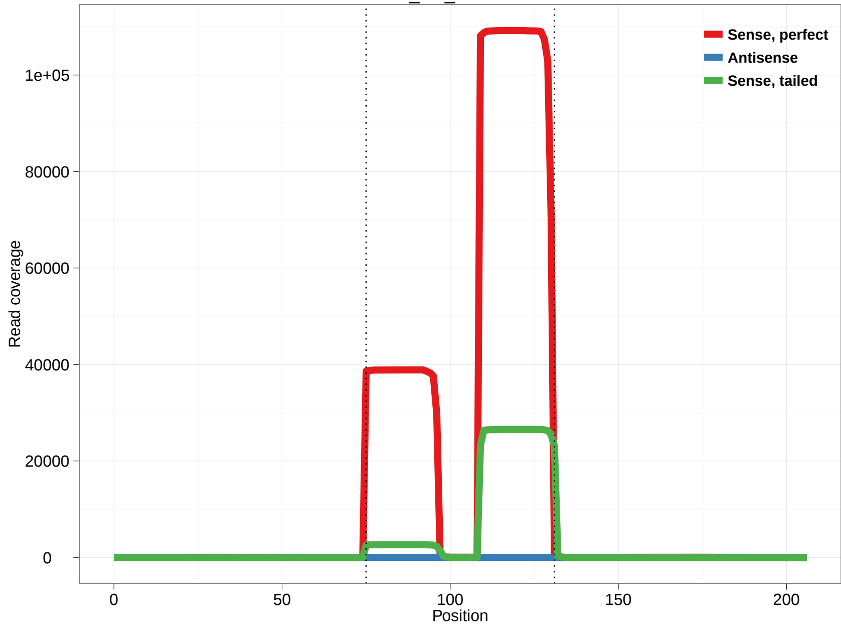
CG6695_in5_dme-mir-1003
