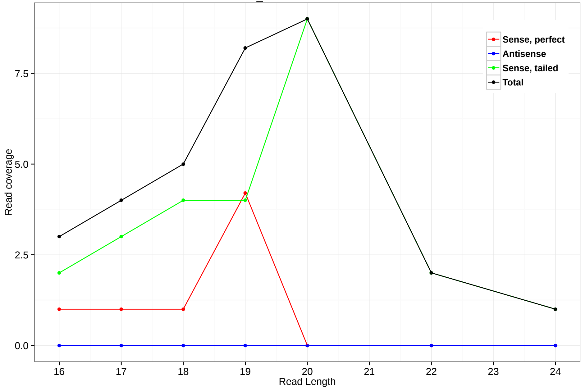
2R_11433348-11433532
