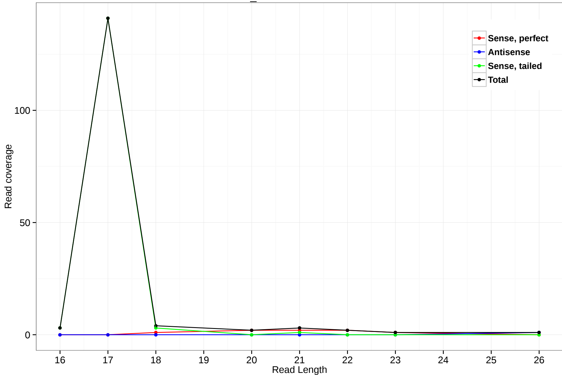
2R_10177847-10178008
