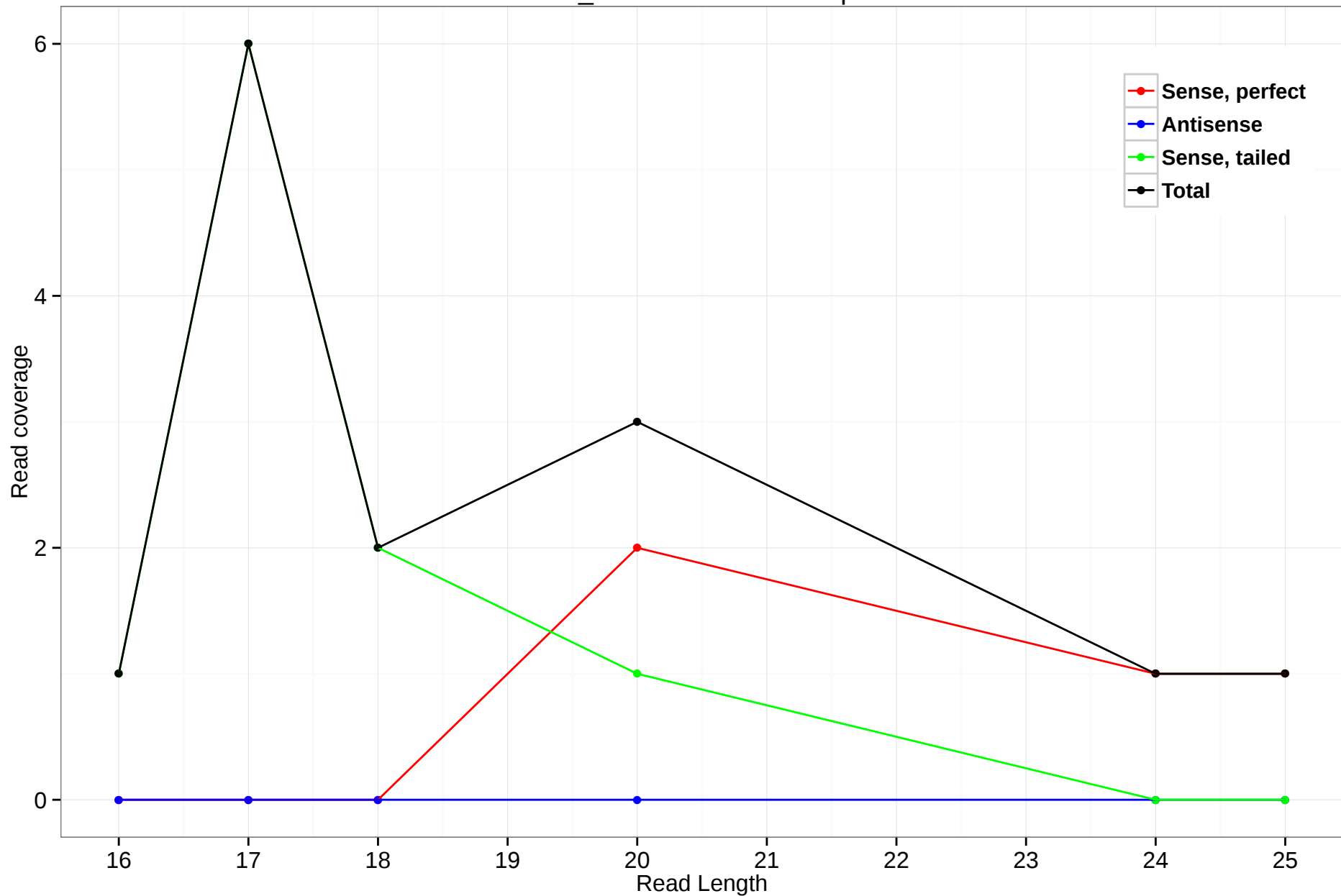
2L_9169083-9169762.3p
